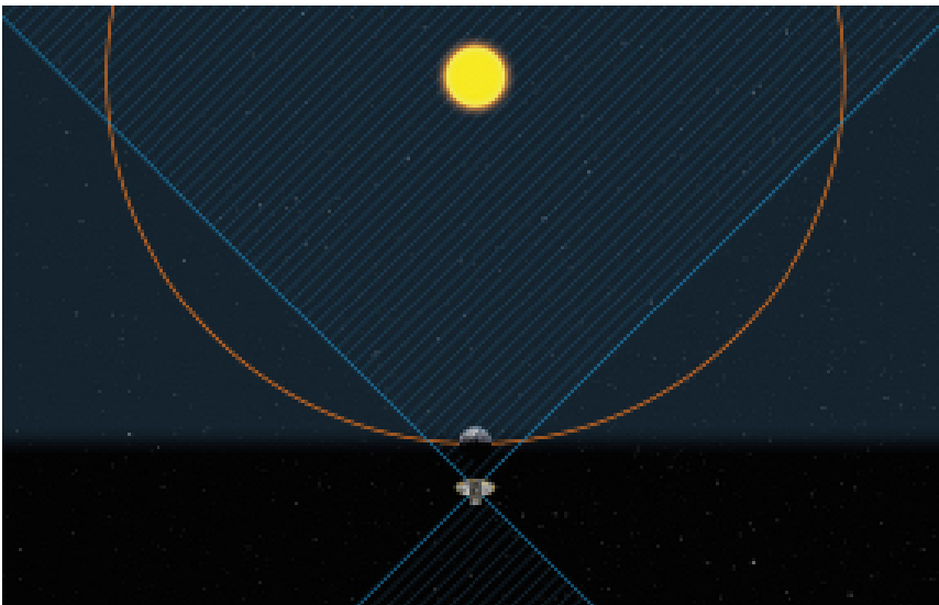
Asteroid search region. Credit: ESA
