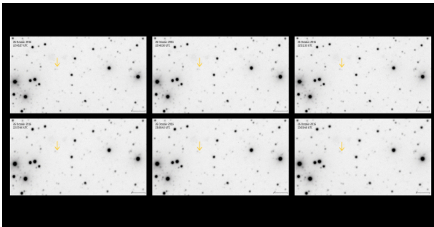
Asteroid Gaia-606 on 26 October 2016. Credit: Observatoire de Haute-Provence & IMCCE
