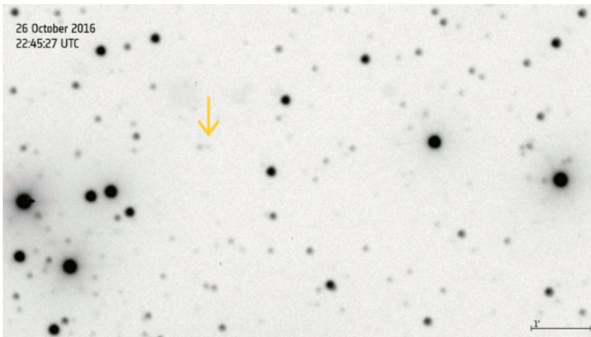
Asteroid Gaia-606 on 26 October 2016. Credit: Observatoire de Haute-Provence & IMCCE
